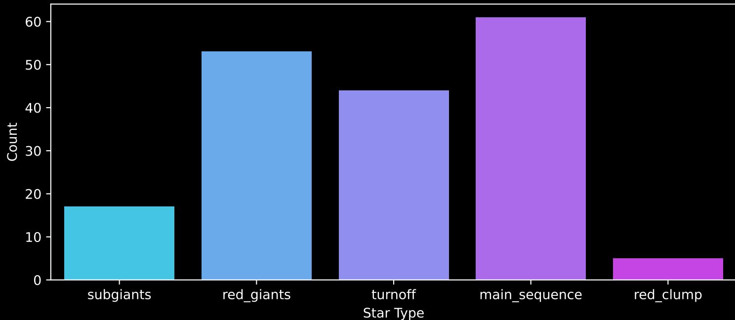
APOGEE DR17 Field: [284-26-O_TESS] Count plot of Star Type
