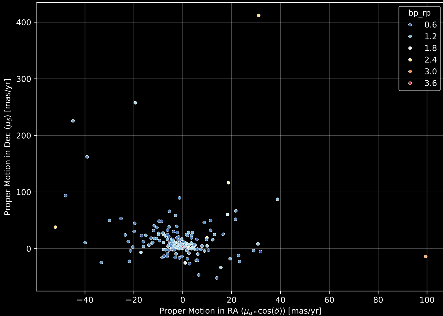
APOGEE DR17 Field: [284-26-O_TESS] Proper Motion Diagram (n= 180)
