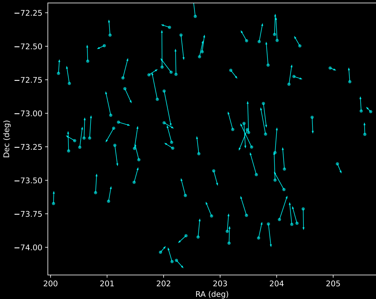
APOGEE DR17 Noise Stream Proper Motion Vectors (n=82)
