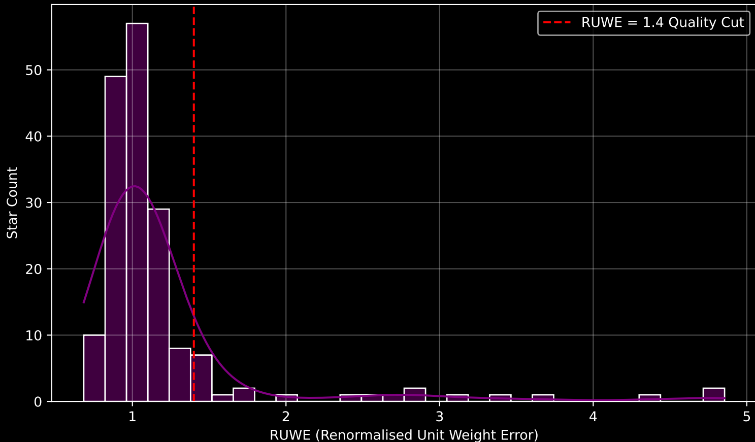
GAPOGEE DR17 Field [284-26-O_TESS] RUWE Distribution (n= 175)
