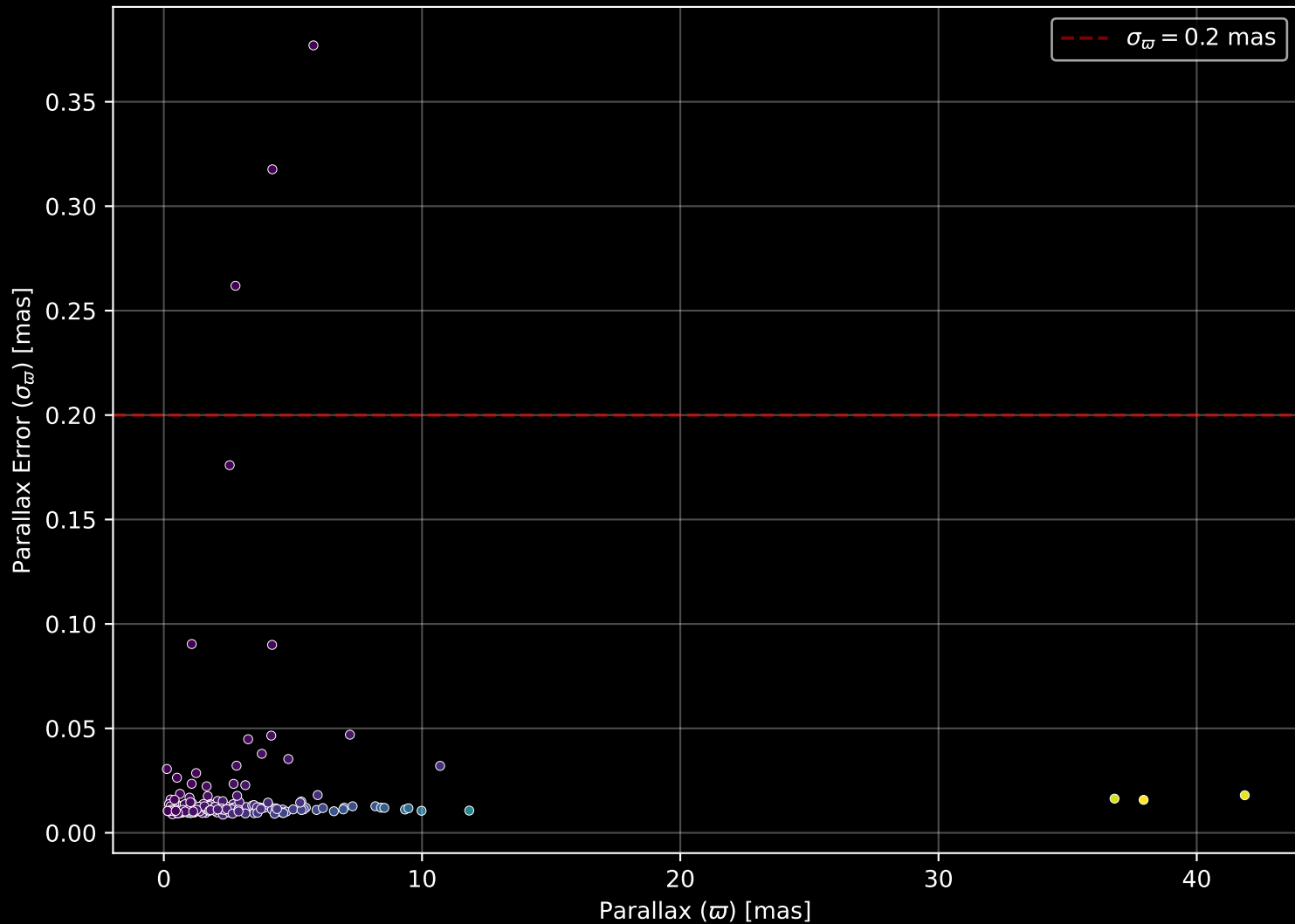
APOGEE DR17 Field: [284-26-O_TESS] Parallax Quality (n= 180)
