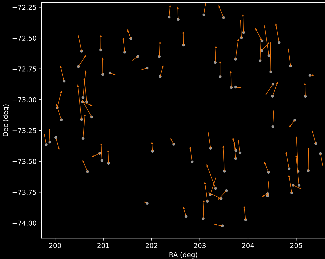
APOGEE DR17 Cluster 2 Proper Motion Vectors (n=81)
