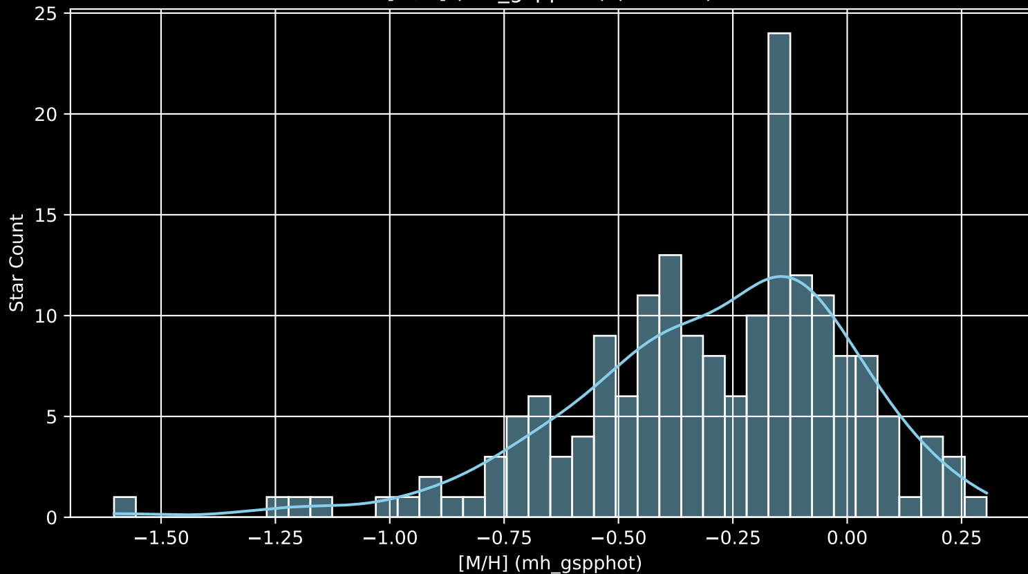
APOGEE DR17 Field: [284-26-O_TESS [M/H] (mh_gspphot) (n= 180)
